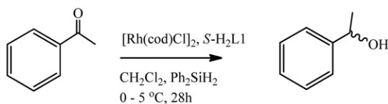
Scheme 2. Catalytic reduction of acetophenone into ( rac )-1-phenylethanol.
