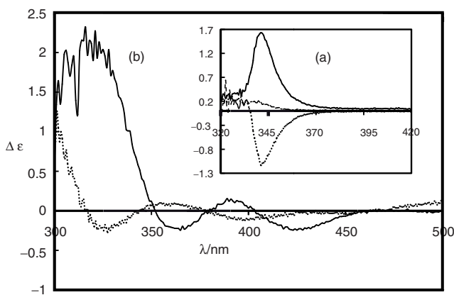
Figure 1. CD spectra of the Schiff bases (a): R -H 2 L1 (solid line, 1.326 \times 10^{-2} \text{ mol dm}^{-3} ); S -H 2 L1 (dot, 1.450 \times 10^{-2} \text{ mol dm}^{-3} ); rac -H 2 L2 (dash, 1.492 \times 10^{-2} \text{ mol dm}^{-3} ); and complexes (b): [\text{Rh}(\eta^4\text{-cod})(\text{R-HL1})] ( 1 ) (solid, 1.193 \times 10^{-2} \text{ mol dm}^{-3} ); [\text{Rh}(\eta^4\text{-cod})(\text{S-HL1})] ( 2 ) (dot, 1.152 \times 10^{-2} \text{ mol dm}^{-3} ) in \text{CHCl}_3 at 20°C.
